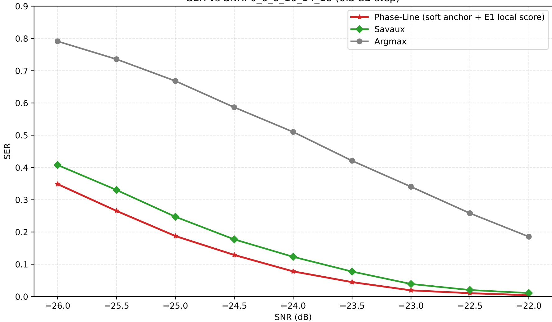
SER vs SNR: 0_0_0_10_14_16 (0.5 dB step)
